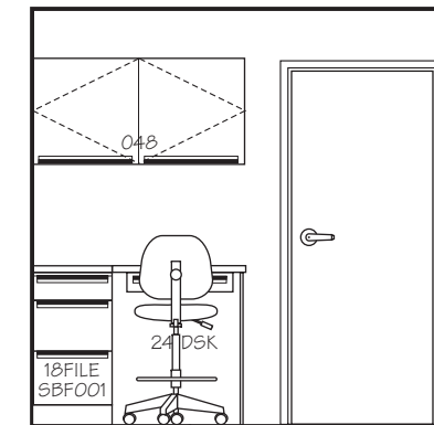
INTAKE-REAR WALL
