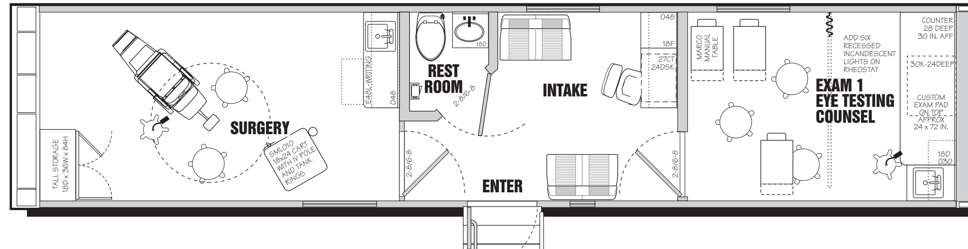
STREET SIDE
